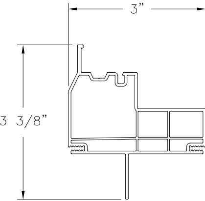
MAIN FRAME (CH9201A) FIN INSTALLATION EXTRUDED RIGID PVC
